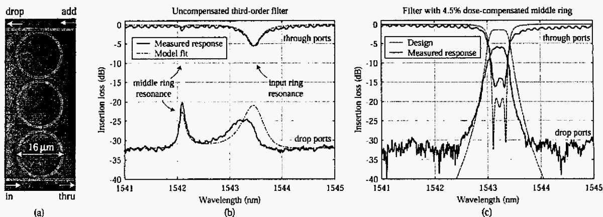
Fig. 3. (a) Micrograph of a compensated filter with 4.5% incremental dose applied to the middle ring; (b) drop- and thru-port responses of 3-ring filter without compensation – experiment (solid) and fit (dotted); (c) drop- and thru-port responses of compensated filter – theory (dash), theory with 15dB/cm waveguide loss (dotted) and experimental (solid).
