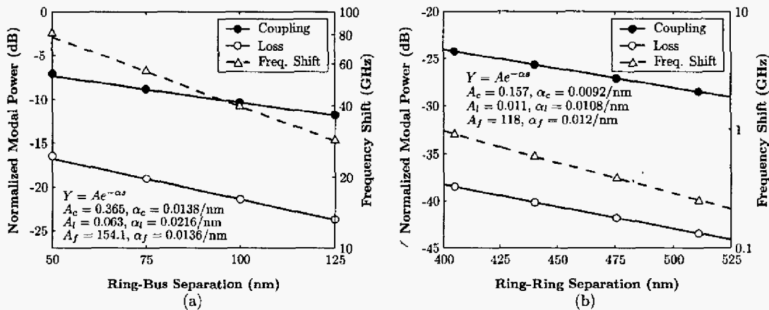
Fig. 2. 3D FDTD determined (a) Ring-Bus and (b) Ring-Ring, coupling, loss, and coupling-induced frequency shifts.
